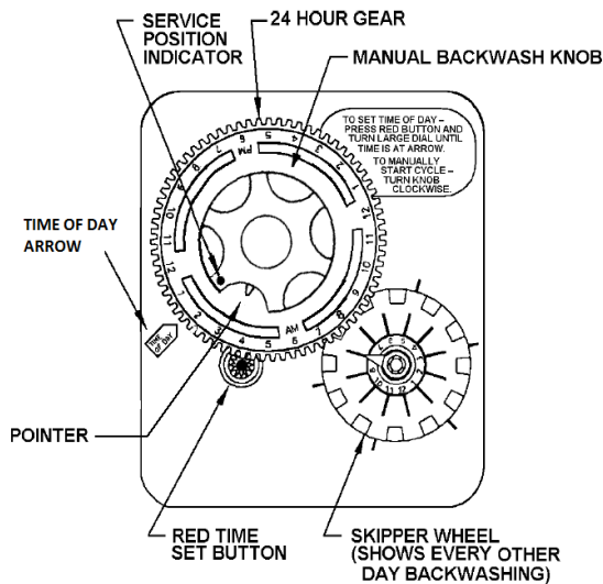
FIGURE 4a: Timer in Service Position
