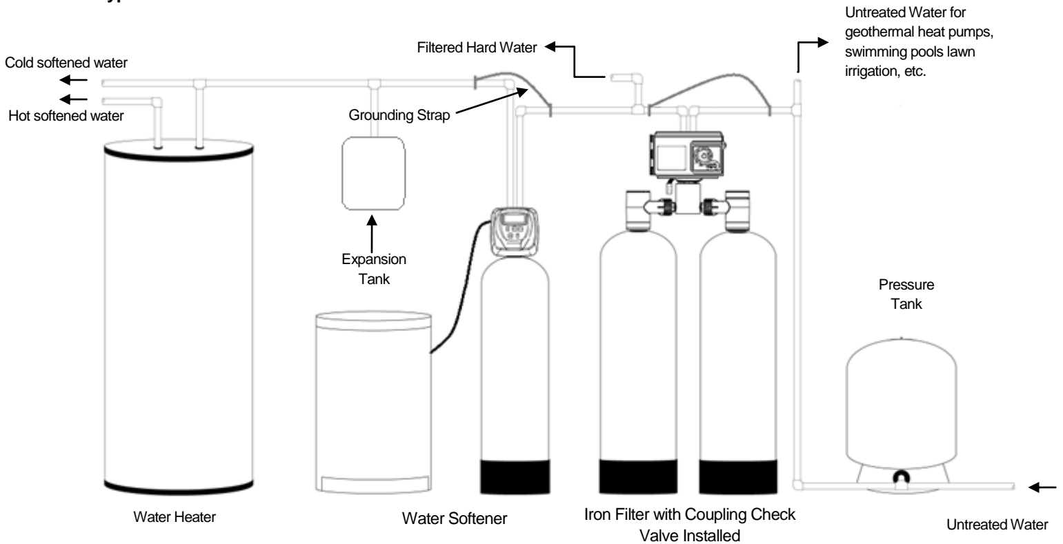
FIGURE 1: Typical Installation
